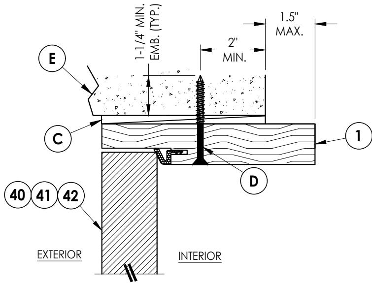
3 7 HORIZONTAL CROSS SECTION Shown Direct to Masonry w/ 6-9/16" jamb
