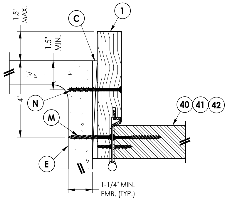
1 7 HORIZONTAL CROSS SECTION Shown Direct to Masonry w/ 6-9/16" jamb
