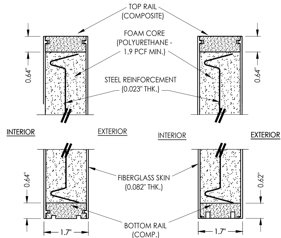
3 VERTICAL CROSS SECTION 2
