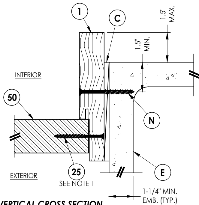
2 7 VERTICAL CROSS SECTION Shown Direct to Masonry w/ 6-9/16" jamb
