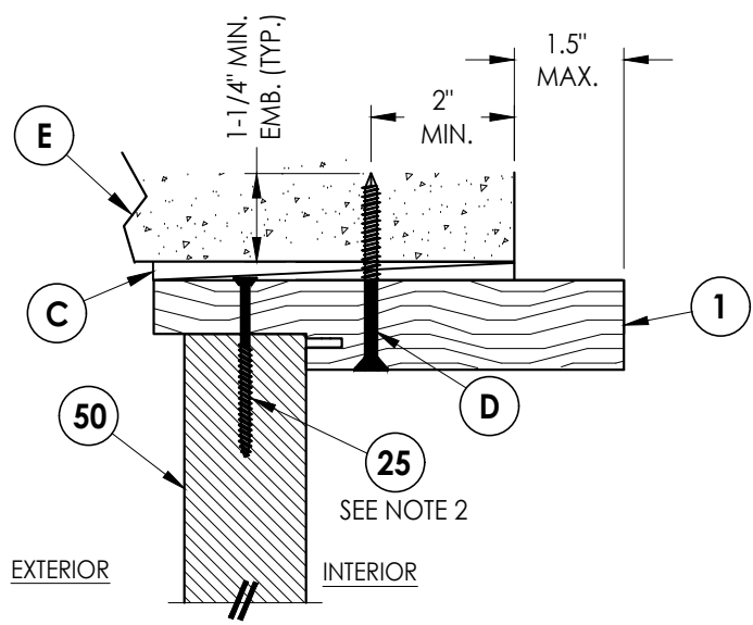
4 7 VERTICAL CROSS SECTION Shown Direct to Masonry w/ 6-9/16" jamb
